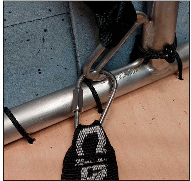
▲ Harness bottom frame attachment
